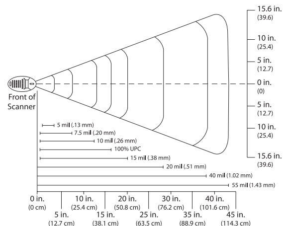
Typical Depth of Field in Inches/Centimeters
